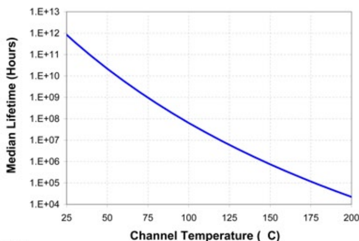
Figure 2. Median Lifetime Curve
