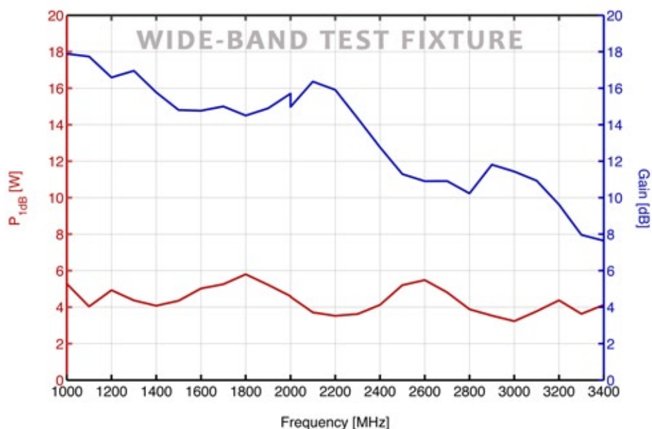
Figure 4: P1dB & Gain versus Frequency
