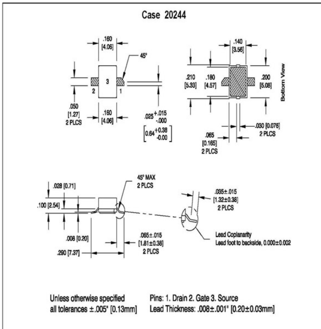
Figure 8. Case Outline Specifications
