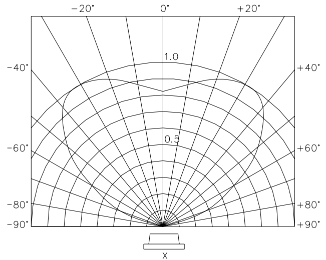
Radiation Diagram
