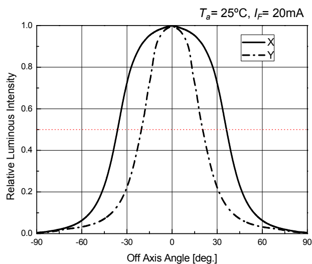
Directivity
