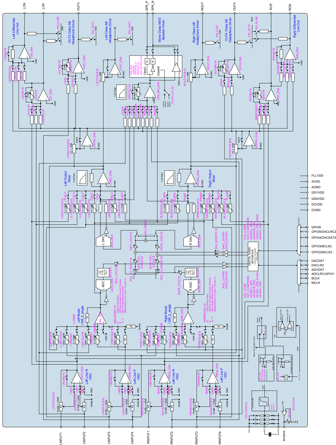
Figure 18 WM8400 Audio Signal Paths
