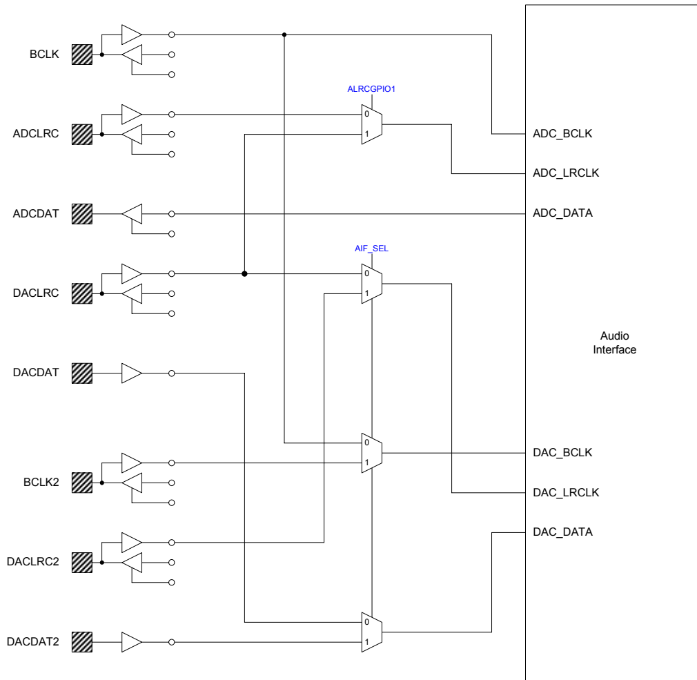
Figure 64 Audio Interface Input Flow
