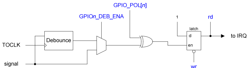
Figure 49 GPIO Function
