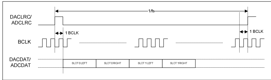
Figure 79 TDM in DSP Mode A
