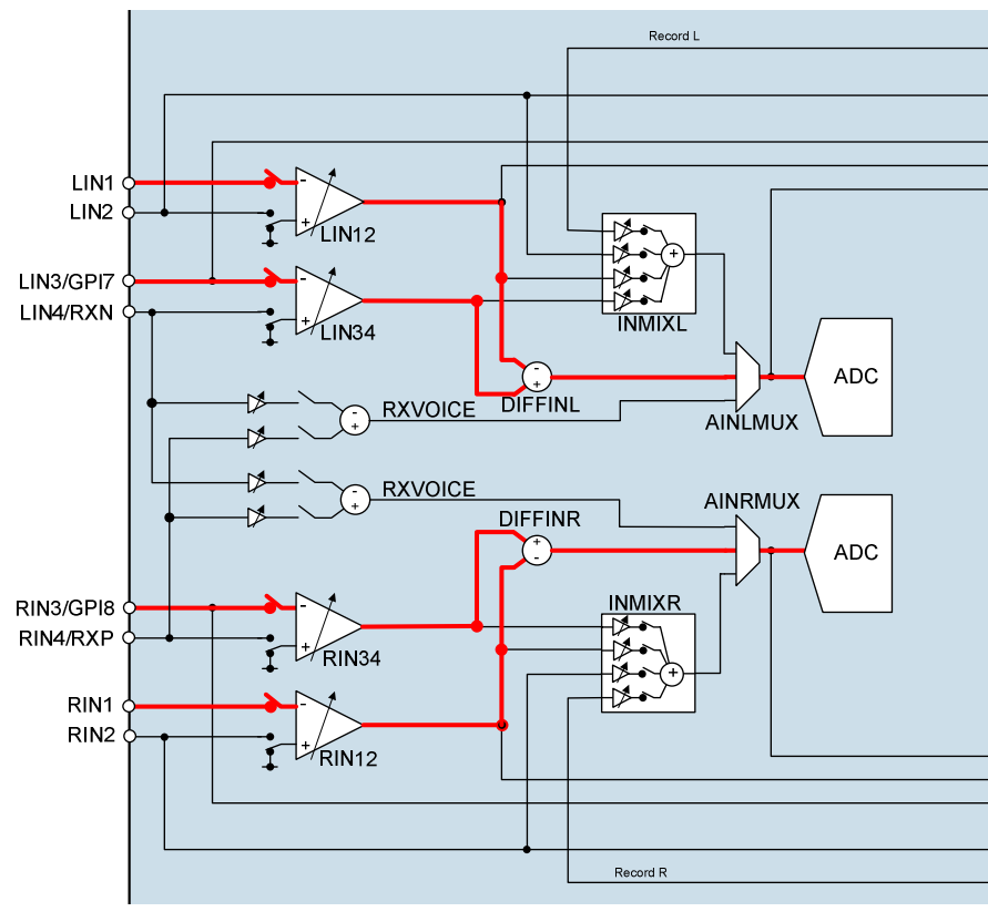
Figure 30 Differential Mode Signal Paths
