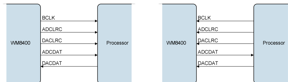
Figure 54 Master Mode
