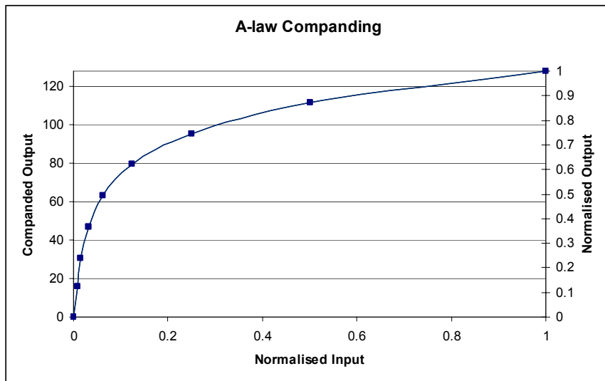
Figure 83 A-Law Comanding
