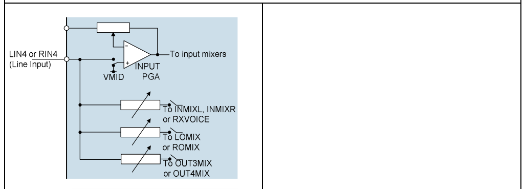
Figure 27 LIN4 or RIN4 as Line Inputs
