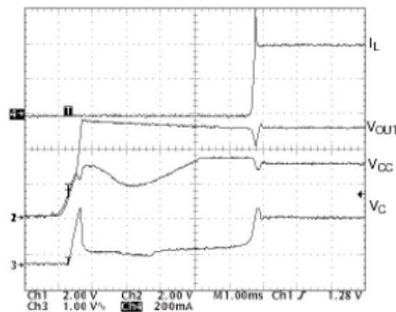
Figure 22. Startup Waveforms of Circuit Shown in the Application Diagram. Load = 400 mA.
