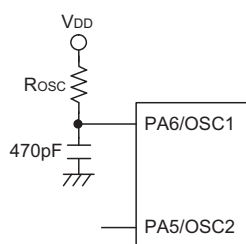
External RC Oscillator – ERC
