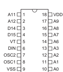
HT692 — 18 DIP-A
