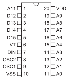
HT614 — 20 DIP-A/SOP-B
