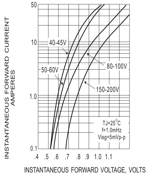
Fig.2- TYPICAL INSTANTANEOUS FORWARD CHARACTERISTIC
