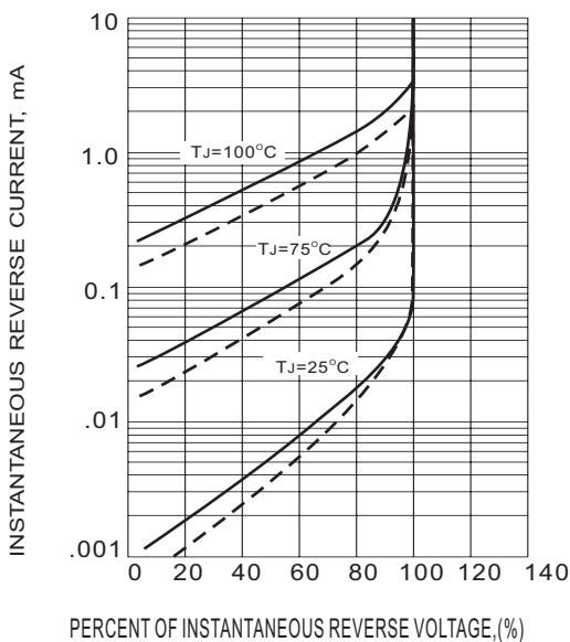
Fig.3- TYPICAL REVERSE CHARACTERISTIC
