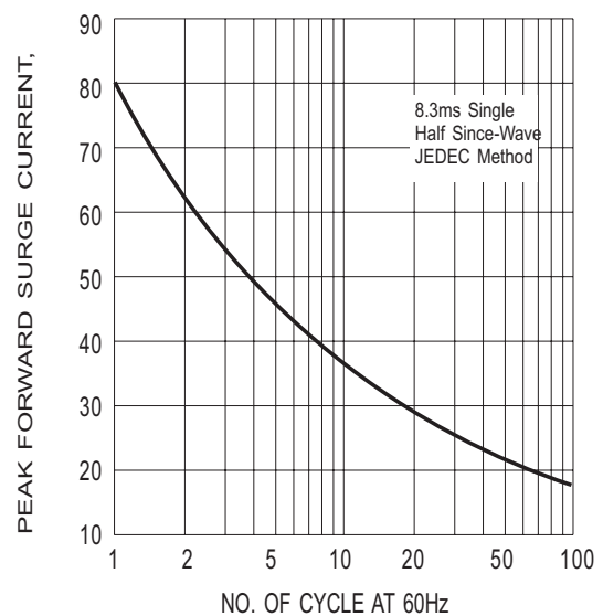
Fig.4- MAXIMUM NON - REPETITIVE SURGE CURRENT
