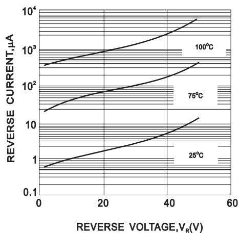
FIG. 2-TYPICAL REVERSE CHARACTERISTIC
