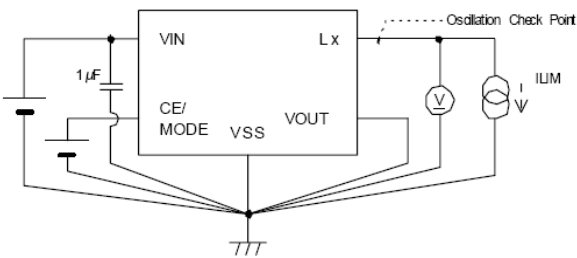
Circuit ⑦
