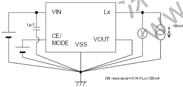
Circuit ⑤
