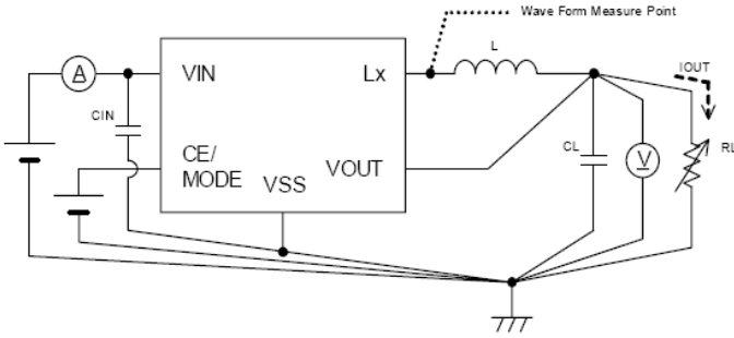
Circuit ③
