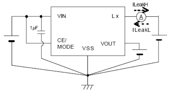
Circuit ⑥
