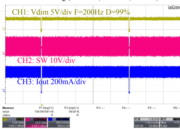
PWM dimming (Vin=12V, L=47uH, 3xLED)
