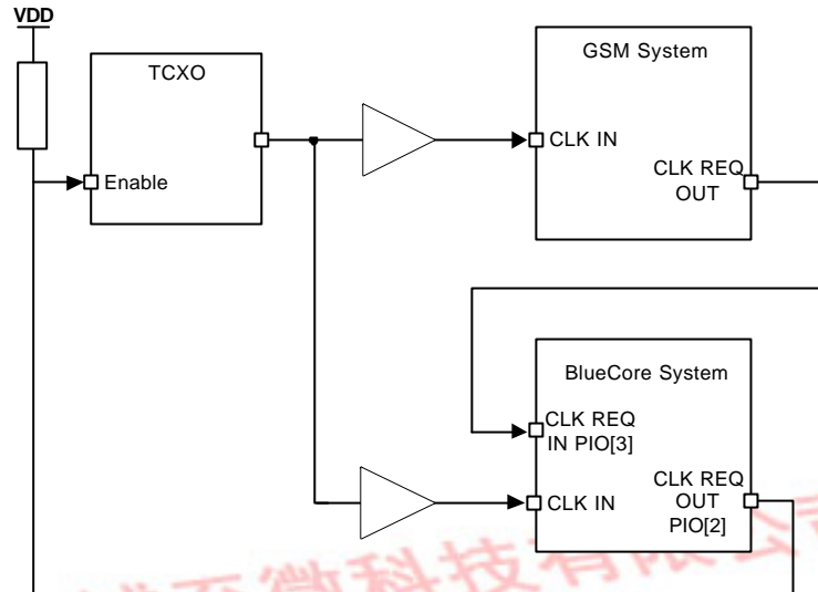
Figure 9.6: Example TCXO Enable OR Function
