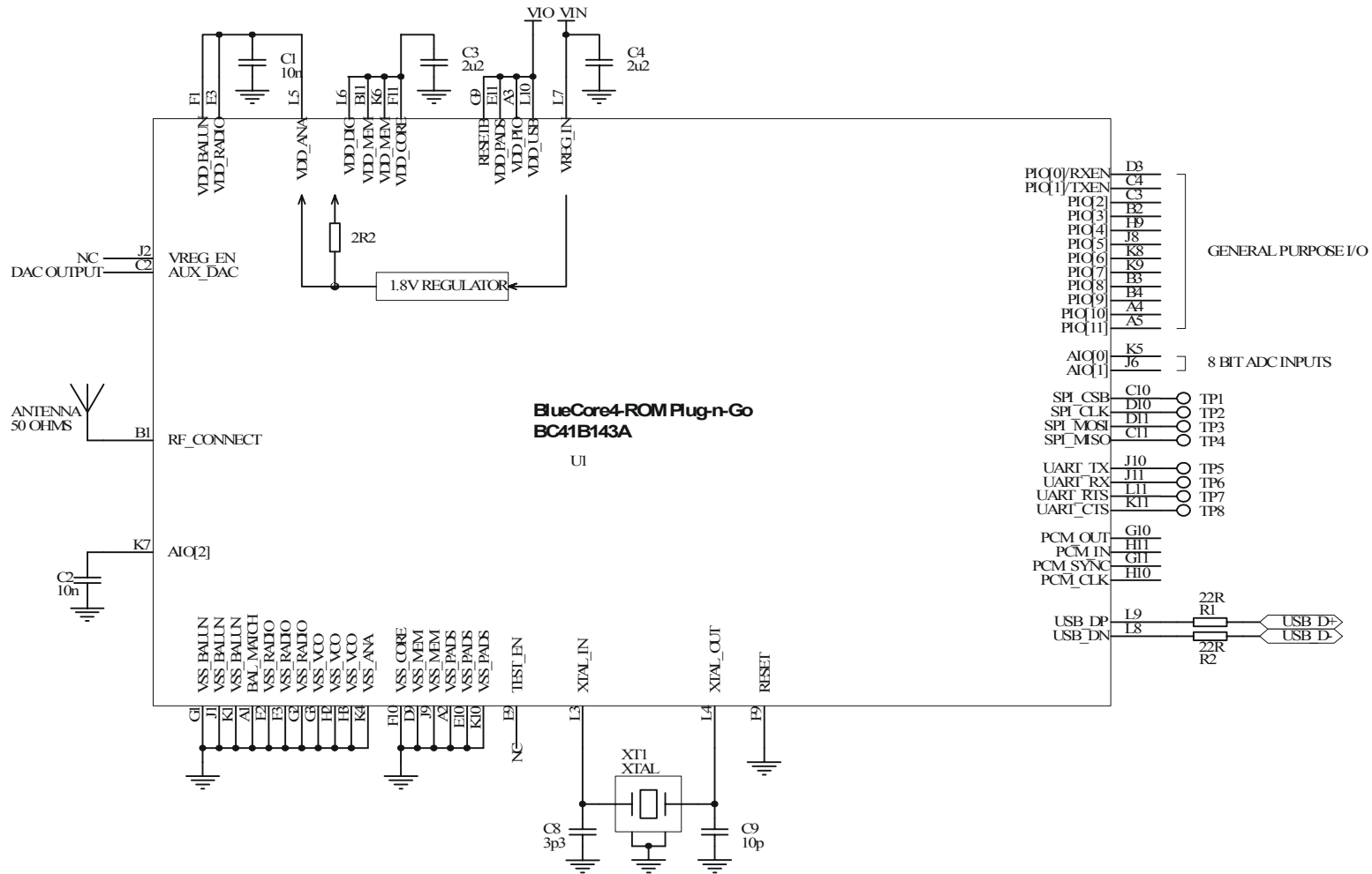
Figure 11.1: Application Circuit for Radio Characteristics Specification
