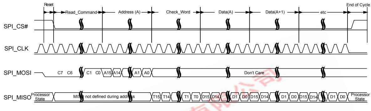
Figure 8.5: SPI Read Operation
