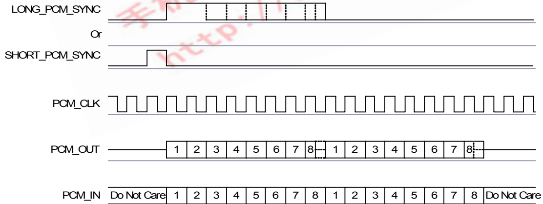
Figure 9.5: Multi-slot Operation with Two Slots and 8-bit Companded Samples
