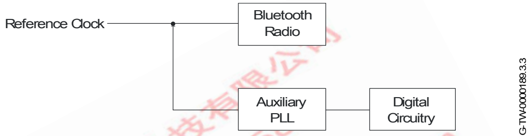
Figure 5.1: Clock Architecture
