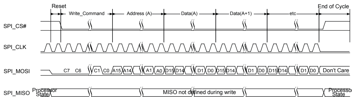
Figure 8.4: SPI Write Operation
