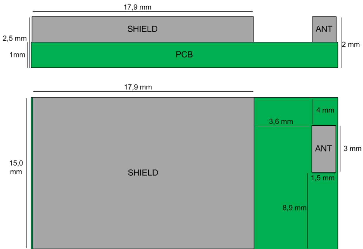
Figure 43: WT32 physical dimensions
