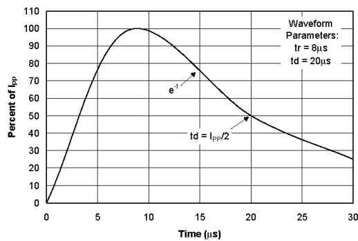
Pulse Waveform
