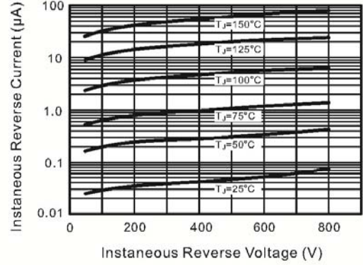
Typical Instantaneous Reverse Characteristics
