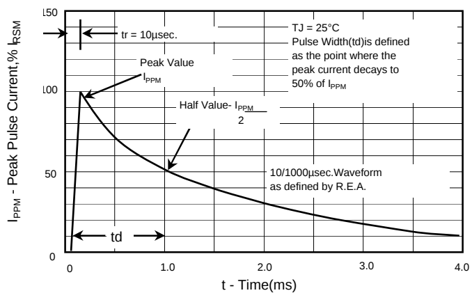
Fig.3 - Pulse Waveform
