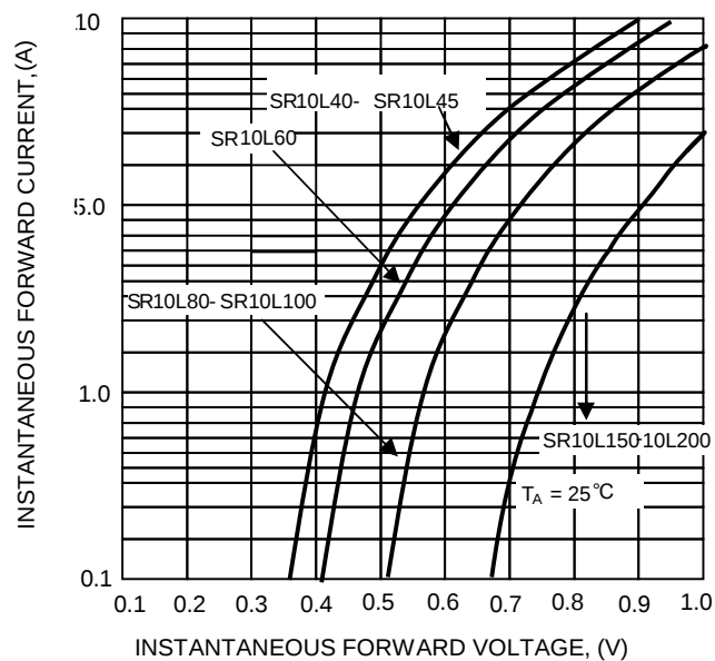
FIG.2-TYPICAL FORWARD CHARACTERISTICS
