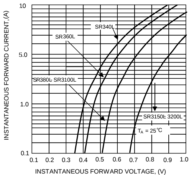
FIG.2-TYPICAL FORWARD CHARACTERISTICS
