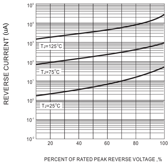
FIG.4TYPICALREVERSE CHARACTERISTIC
