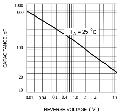
Fig. 4-TYPICAL JUNCTION CAPACITANCE
