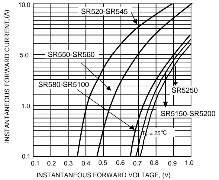
FIG.2-TYPICAL FORWARD CHARACTERISTICS
