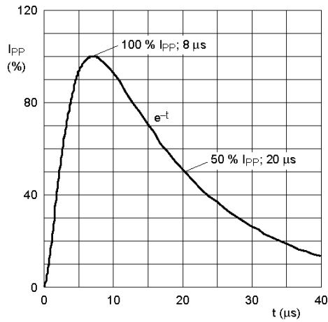
8/20 \mu s pulse waveform according to IEC 61000-4-5
