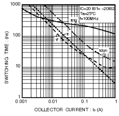
Fig. 6 Switching time
