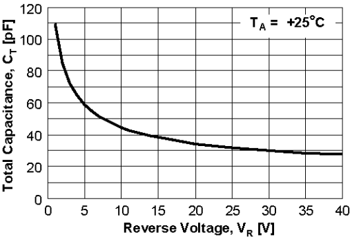
Total Capacitance
