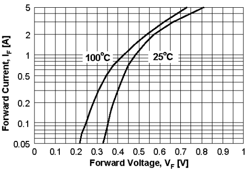
Forward Voltage Characteristics
