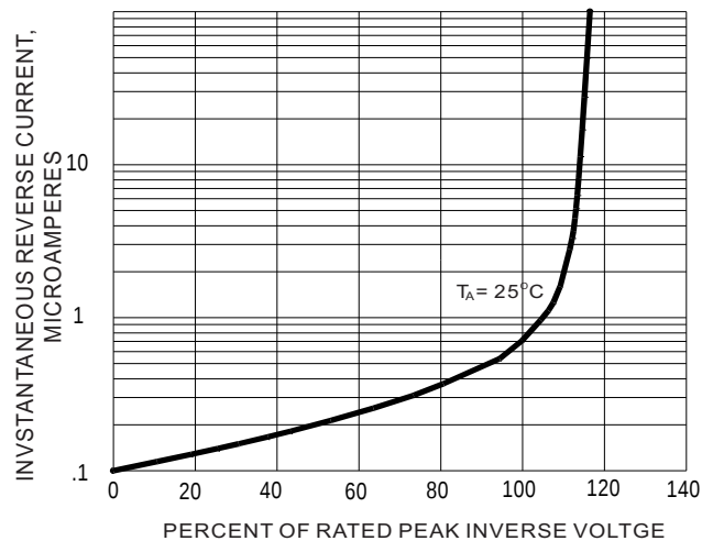
FIG.4-TYPICAL REVERSE CHARACTERISTICS
