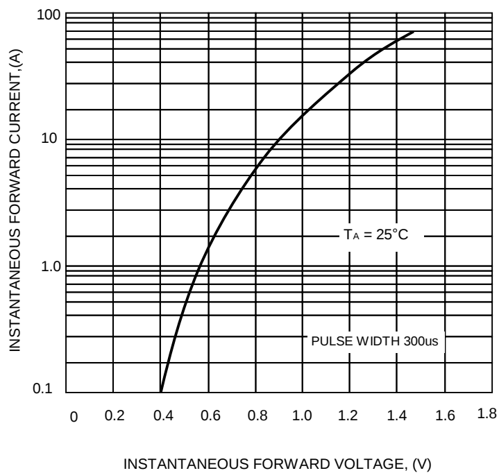
FIG.2-TYPICAL FORWARD CHARACTERISTICS
