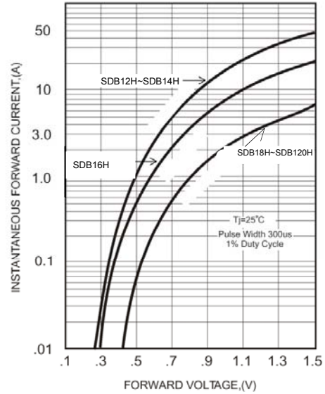
FIG.2-TYPICAL FORWARD CHARACTERISTICS
