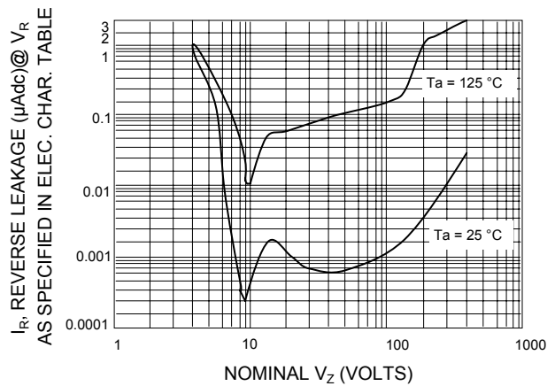
FIG. 4 - TYPICAL REVERSE LEAKAGE
