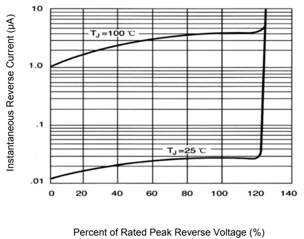
Figure 4. Typical Reverse Characteristics Per Element
