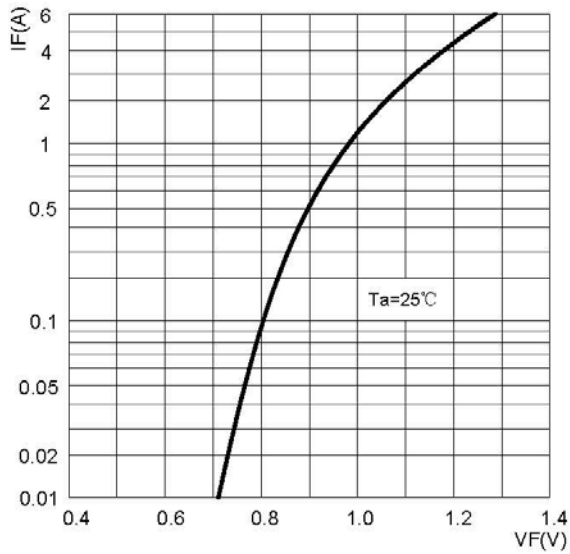
Forward Voltage
