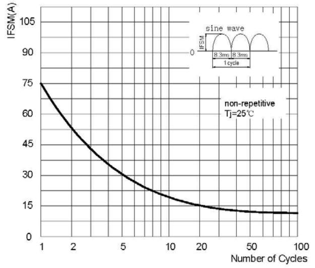
Surge Forward Current Capacity
