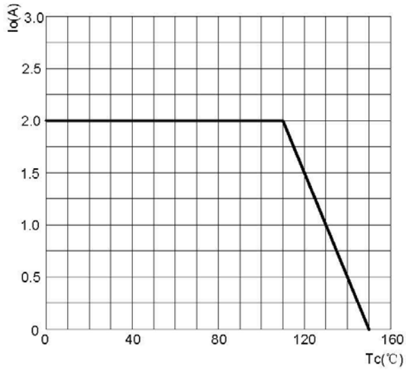
Io-Tc Curve
