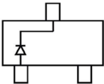
BAS40W MARKING: 43•
