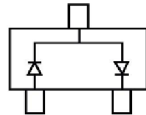
BAS40W-04 MARKING: 44
