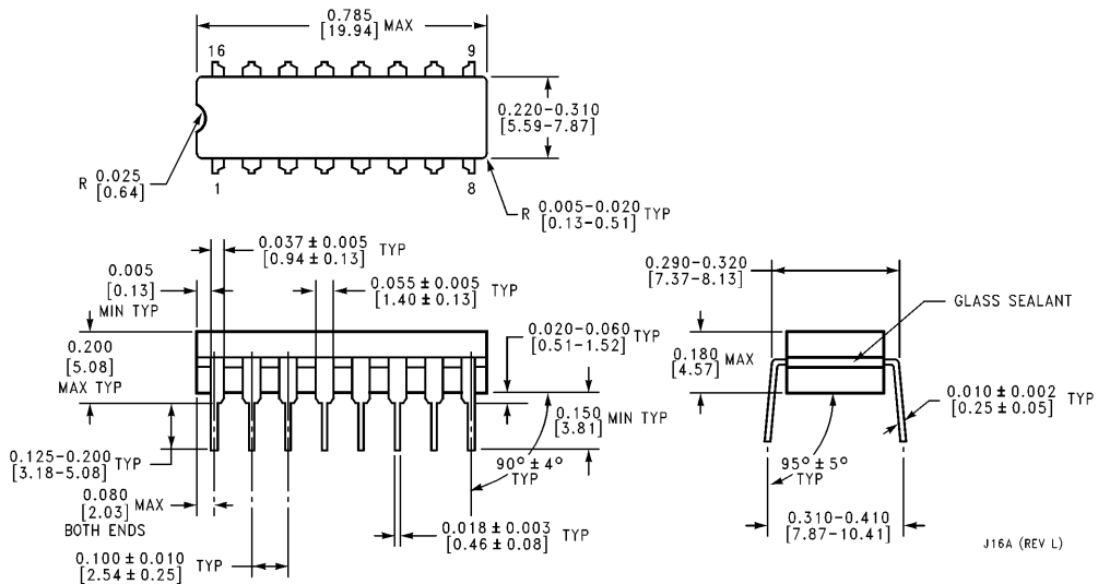
Ceramic Dual-In-Line Package (J) Order Number CD4099BMJ or CD4099BCJ NS Package Number J16A
