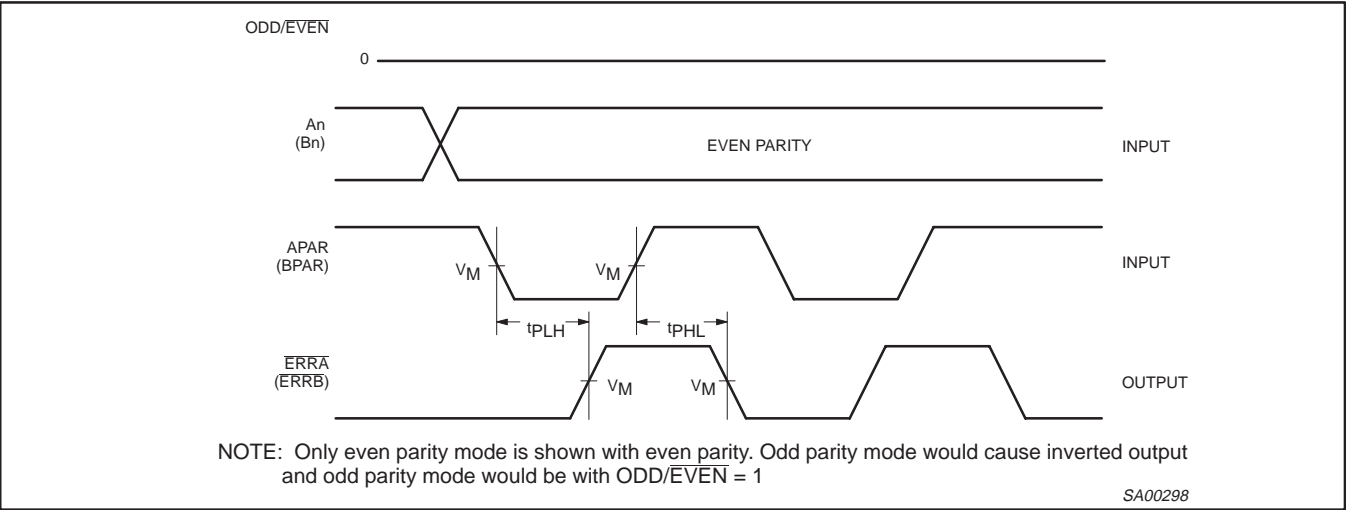
Waveform 6. Propagation Delay, APAR to ERR \bar{A} or BPAR to ERR \bar{B}
