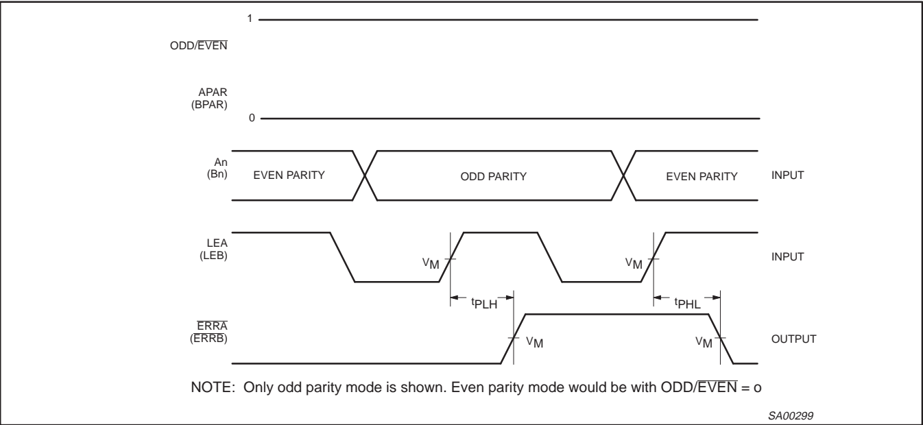
Waveform 7. Propagation Delay, LEA to ERR \bar{A} or LEB to ERR \bar{B}
