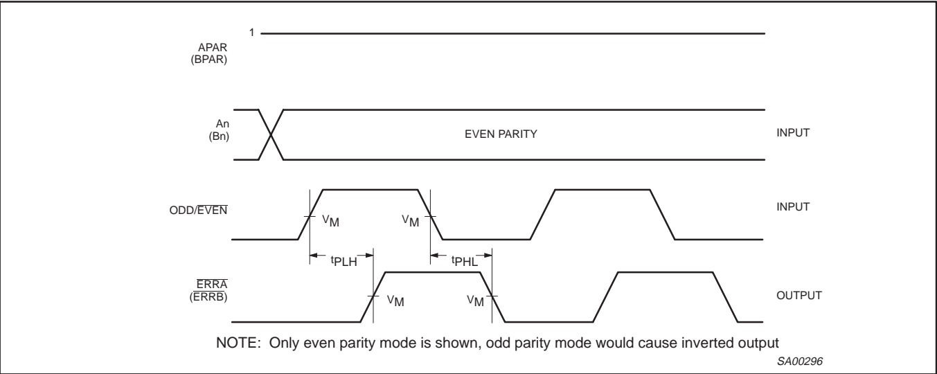
Waveform 4. Propagation Delay, ODD/EVEN to ERRA or ODD/EVEN to ERB
