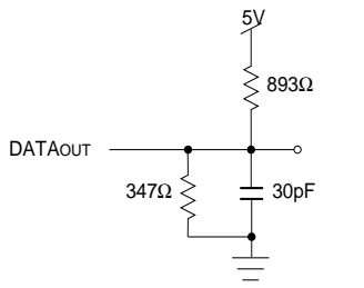
Figure 1. AC Output Test load.
