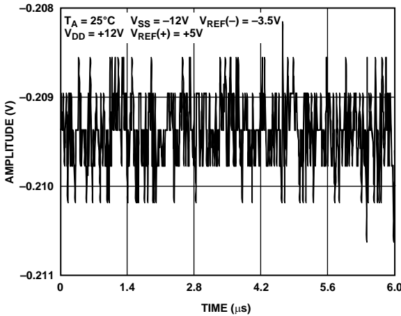
Figure 16. Digital Feedthrough
