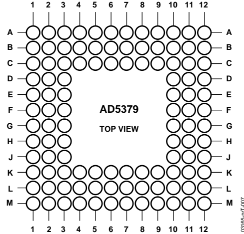
Figure 7. Pin Configuration
