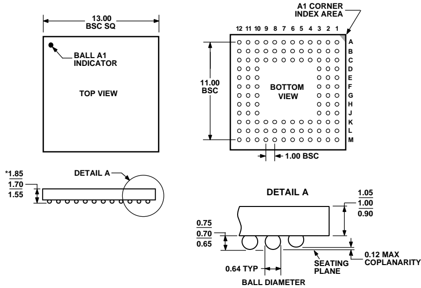
Figure 23. 108-Lead Chip Scale Ball Grid Array [CSPBGA] (BC-108)
