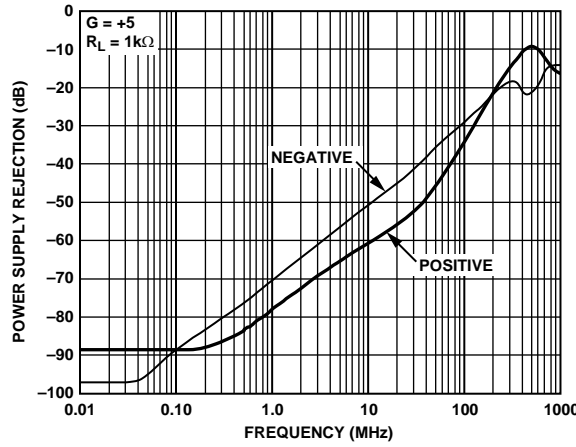
Figure 50. Power Supply Rejection vs. Frequency
