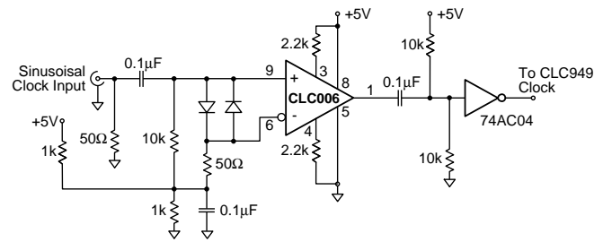
Figure 2: Clock Generation
