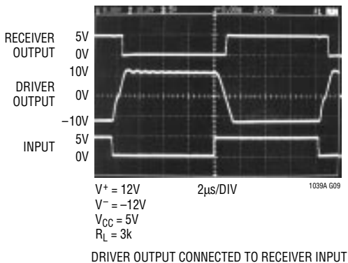
Output Waveforms
