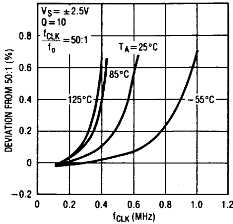
Graph 13. Mode 1: ( f_{CLK}/f_o ) vs f_{CLK} and Temperature
