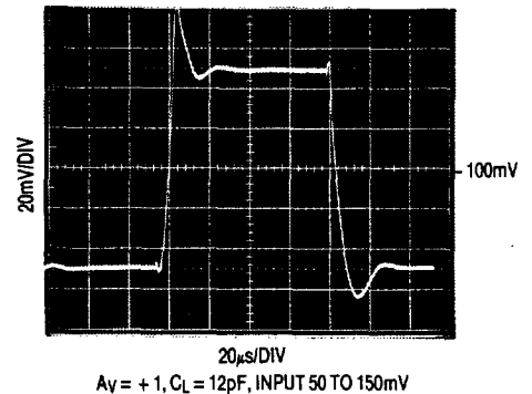
Small Signal Transient Response VS = 5V, 0V
