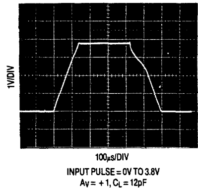
Large Signal Transient Response VS = 5V, 0V
