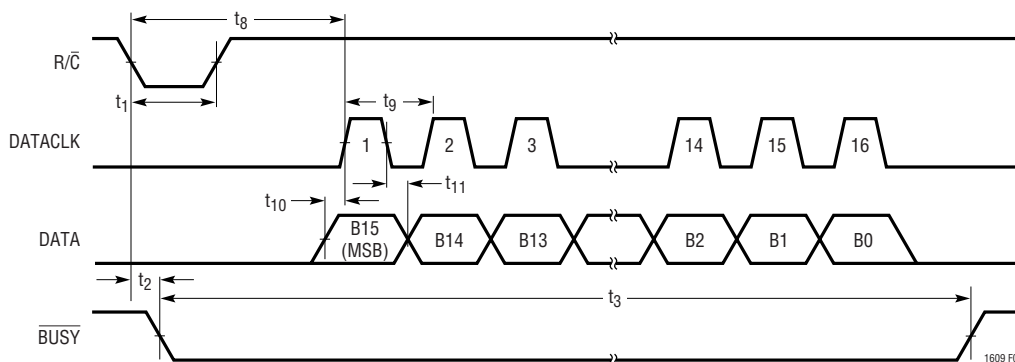
Figure 8. Serial Data Timing Using Internal Clock ( \overline{\text{CS}} , EXT/ \overline{\text{INT}} and TAG Tied Low)
