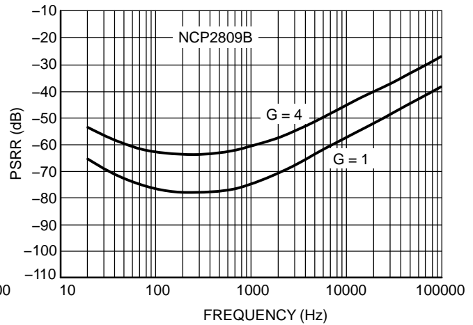
Figure 37. PSRR – Input Grounded with 10 \Omega V_p = 5.0\text{ V} , V_{\text{ripple}} = 200\text{ mV pk-pk} , R_L = 16\ \Omega , G = 1\ (0\text{ dB}) and G = 4\ (12\text{ dB})
