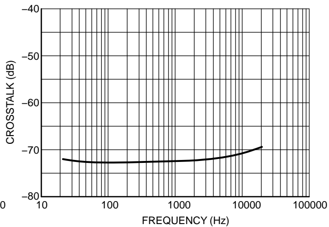
Figure 25. Crosstalk V_p = 2.4 \text{ V} , R_L = 32 \Omega , P_{out} = 10 \text{ mW}
