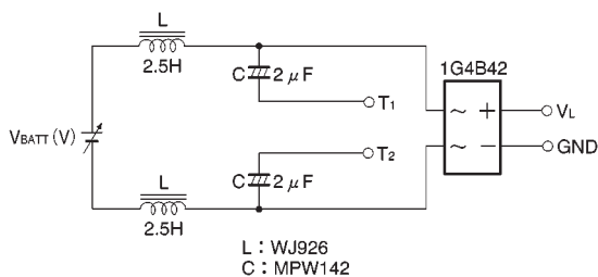
Fig. 15 Trunk circuit
