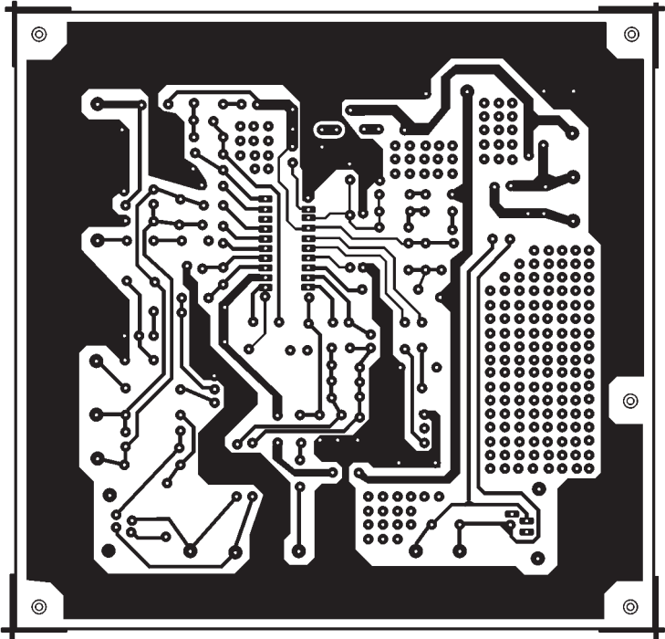
Soldering surface
