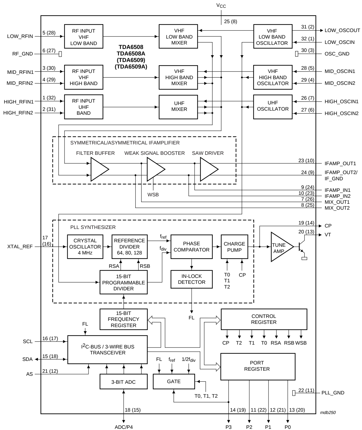
Fig.1 Block diagram.
