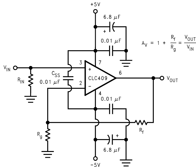
FIGURE 1. Recommended Non-Inverting Gain Circuit
