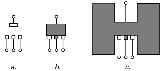
Figure 4. PCB Layouts
