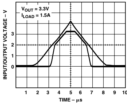
TPC 8. Power-Up/Power-Down Current
