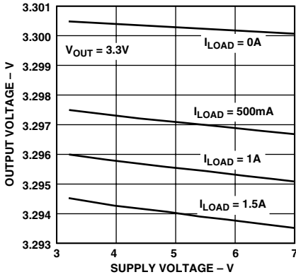
TPC 1. Output Voltage vs. Supply Voltage
