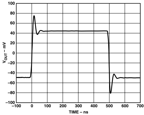
TPC 2. 100 mV Step Response; G = +5 , V_S = \pm 6 V, R_L = 25 \Omega , Single-Ended
