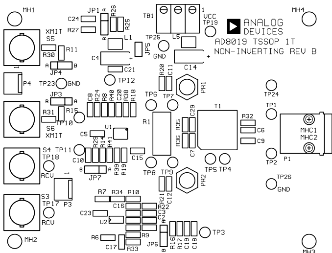
Figure 10. TSSOP Evaluation Board Silkscreen Top
