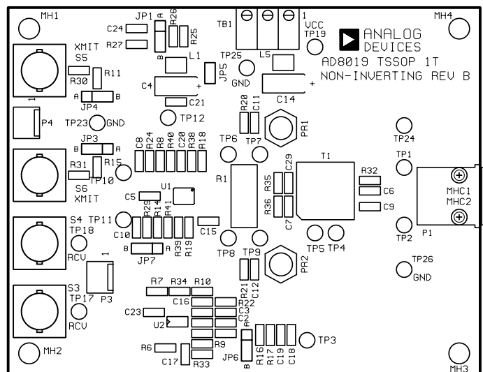
Figure 16. Assembly Top
