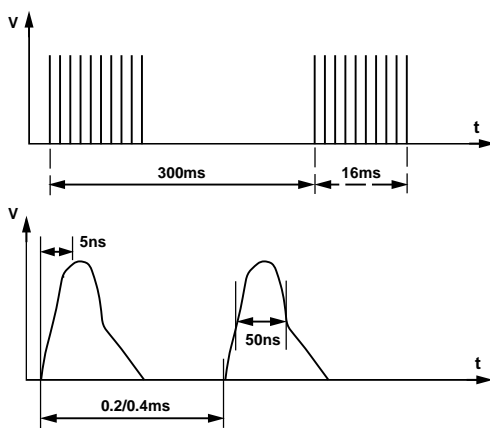
Figure 20. IEC1000-4-4 Fast Transient Waveform
