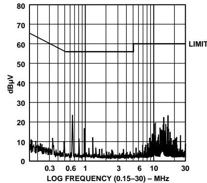
Figure 24. Conducted Emissions
