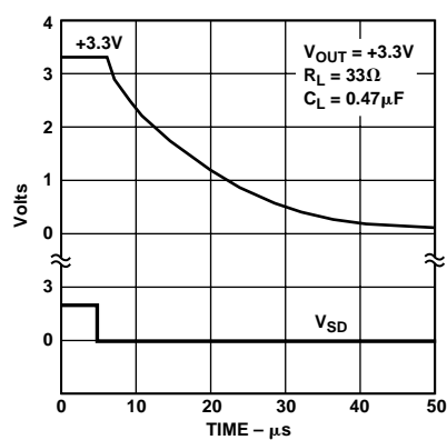
Figure 17. Turn Off
