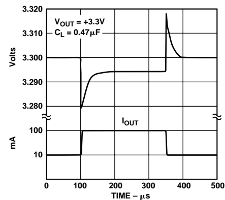
Figure 13. Load Transient
