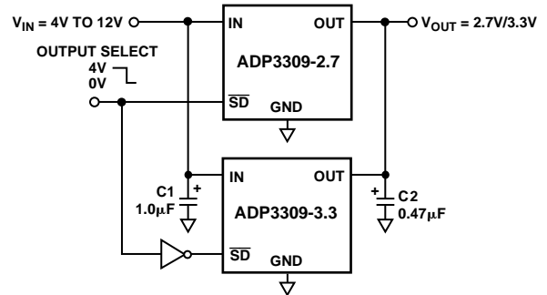
Figure 21. Crossover Switch
