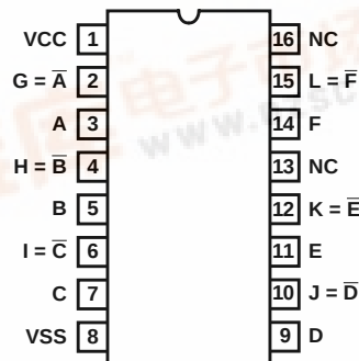
CD4049UBMS TOP VIEW
